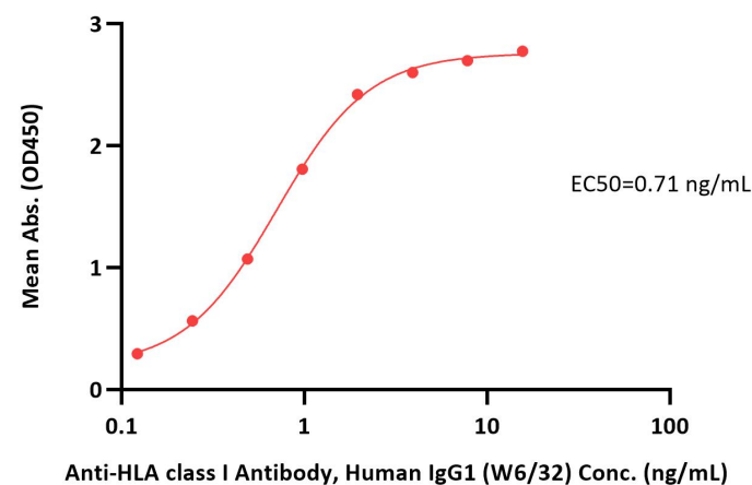
PE-Labeled Human HLA-A*11:01&B2M&KRASG12V (VVVGAVGVGK) Tetramer Protein ELISA 0.1 µg of PE-Labeled Human HLA-A*11:01&B2M&KRASG12V (VVVGAVGVGK) Tetramer Protein per well
